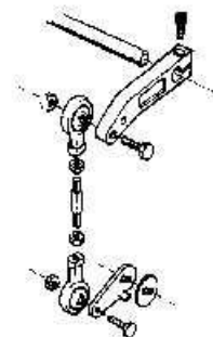
6061-T6 Hex bar with forged rod ends
